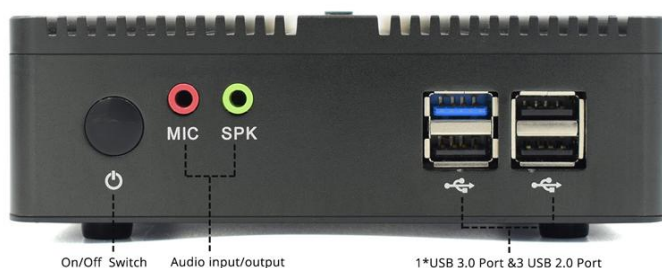
On/Off Switch Audio input/output 1*USB 3.0 Port & 3 USB 2.0 Port
